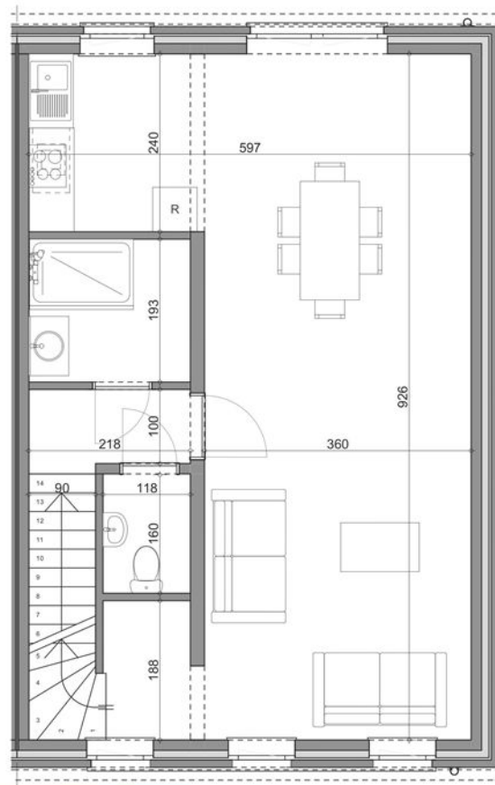
Plan rez - Lot n° 5 -
