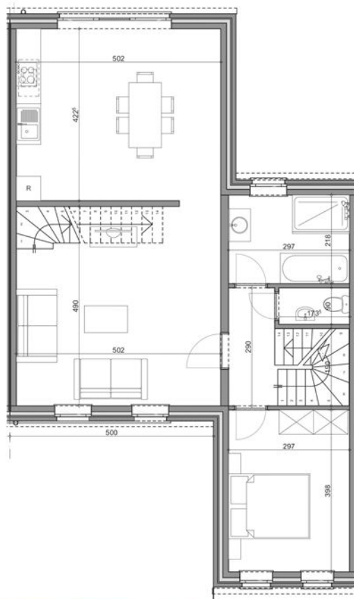
Plan rez - Lot n° 4 -
