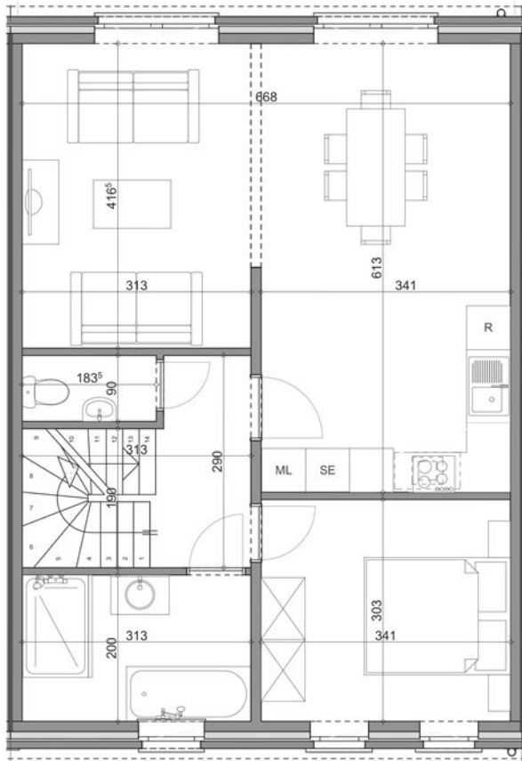
Plan rez - Lot n° 2 -
