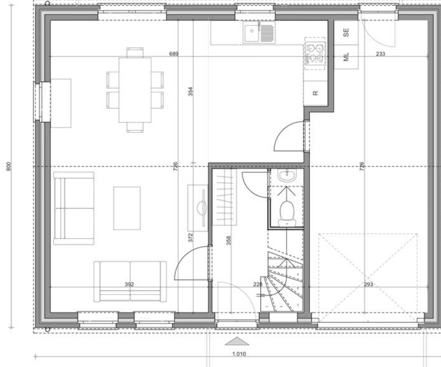
Plan rez - lot n° 2 -
