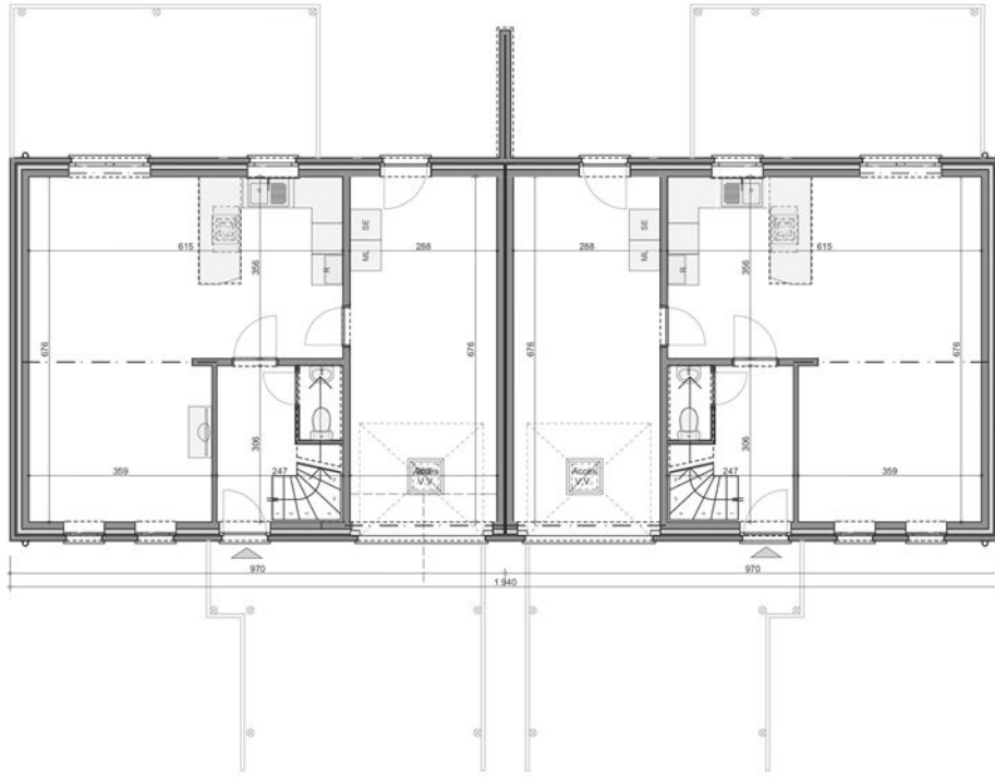
Plan rez - Lot n° 1 -
